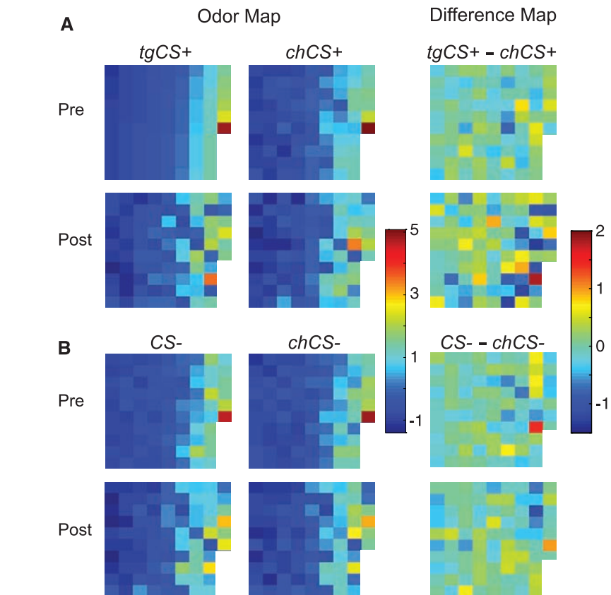
Fig. 3. Spatial maps of posterior piriform activity from one subject. Condition-specific spatial patterns (left two columns) for the CS+ pair (A), but not the CS- pair (B), diverged after conditioning. Difference maps between odorant pairs (right column) highlight the selective differentiation within the CS+ pair after conditioning. Each square in the grid represents fMRI signal intensity from a different piriform voxel ( n = 86 voxels), arranged in columns from top left to bottom right, in ascending order of signal intensity for tgCS+ in the preconditioning phase.
